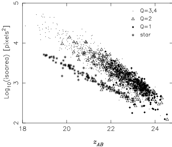
FIG. 12.— Apparent object size (ACS isophotal image area) vs. apparent z magnitude measured in the outermost aperture ( 3'' ) on ACS images (Giavalisco et al. 2004) for the 1981 sources observed in our redshift survey. Different symbols distinguish objects with secure redshifts ( Q = 3, 4 ), uncertain redshifts ( Q = 2 ), no measured redshifts ( Q = 1 ), and stars ( Q = -1 ).
